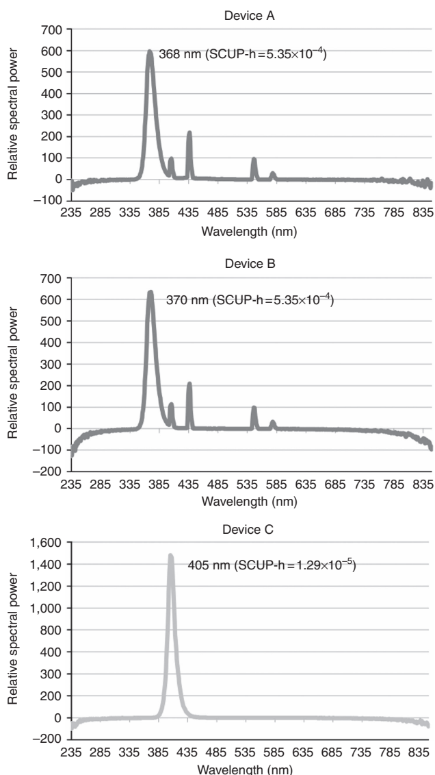
Figure 1. UV nail lamp spectral power distribution by device. Note: According to the manufacturer, the negative spectral irradiance values are due to fluctuations in electronic noise, where noise in the dark may be slightly higher than the noise acquired during the sample measurement at a given wavelength. In that case, if there is no signal in the given region, that value appears negative.
